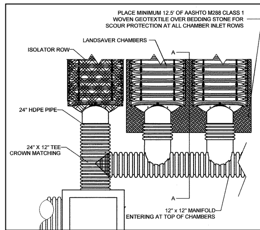
Underground Storage Chamber Details
