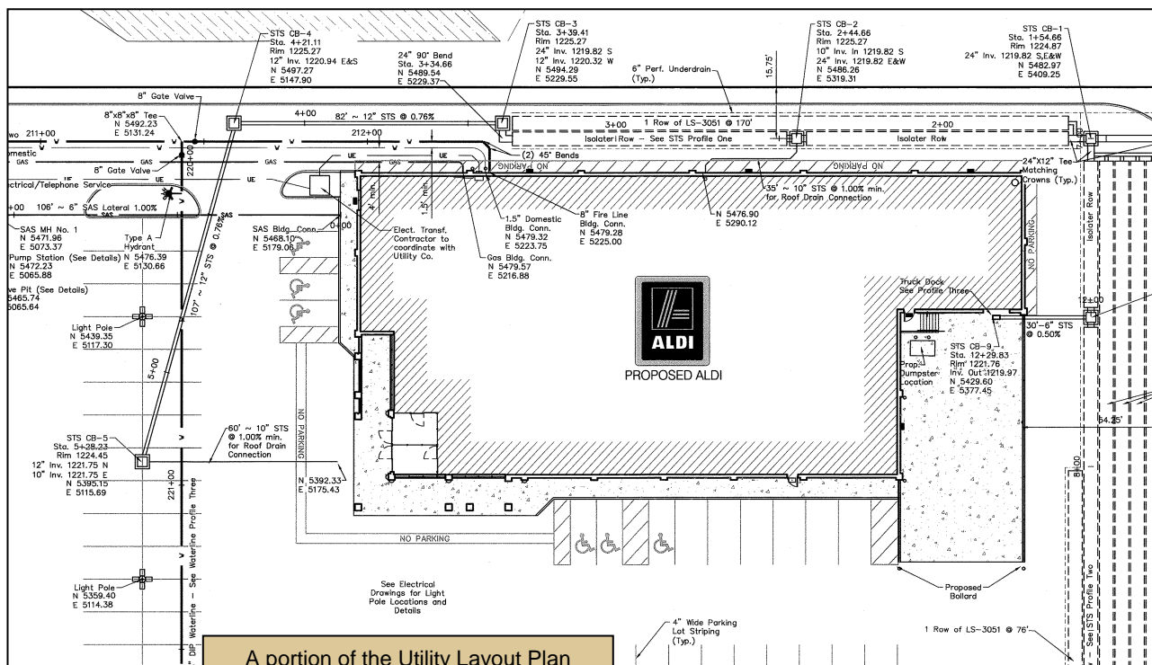
A portion of the Utility Layout Plan
