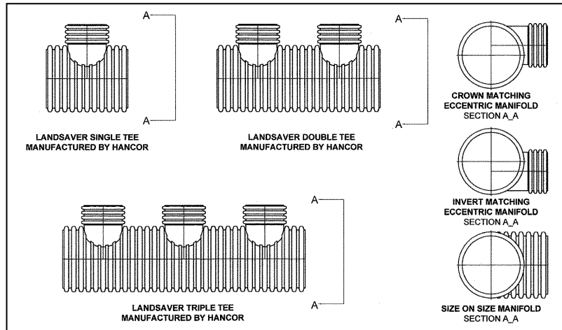
Underground Storage Chamber Details
