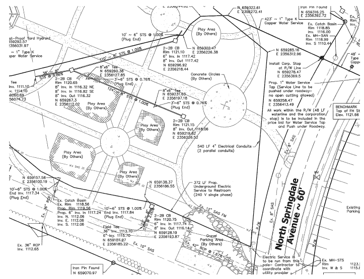
A portion of the Utility Location Plan
