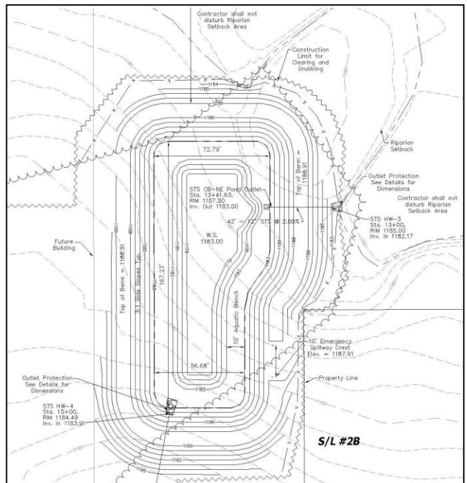
Grading Detail of a stormwater retention pond on the site plan
