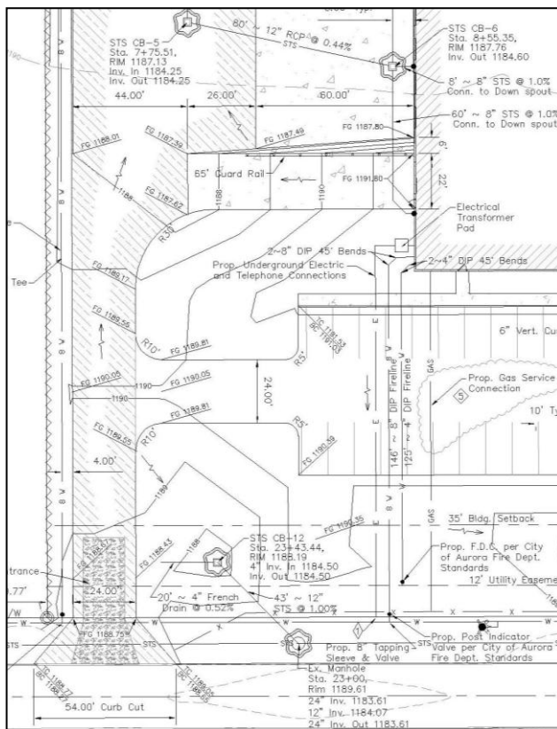
A portion of the site plan showing Grading and Utility details
